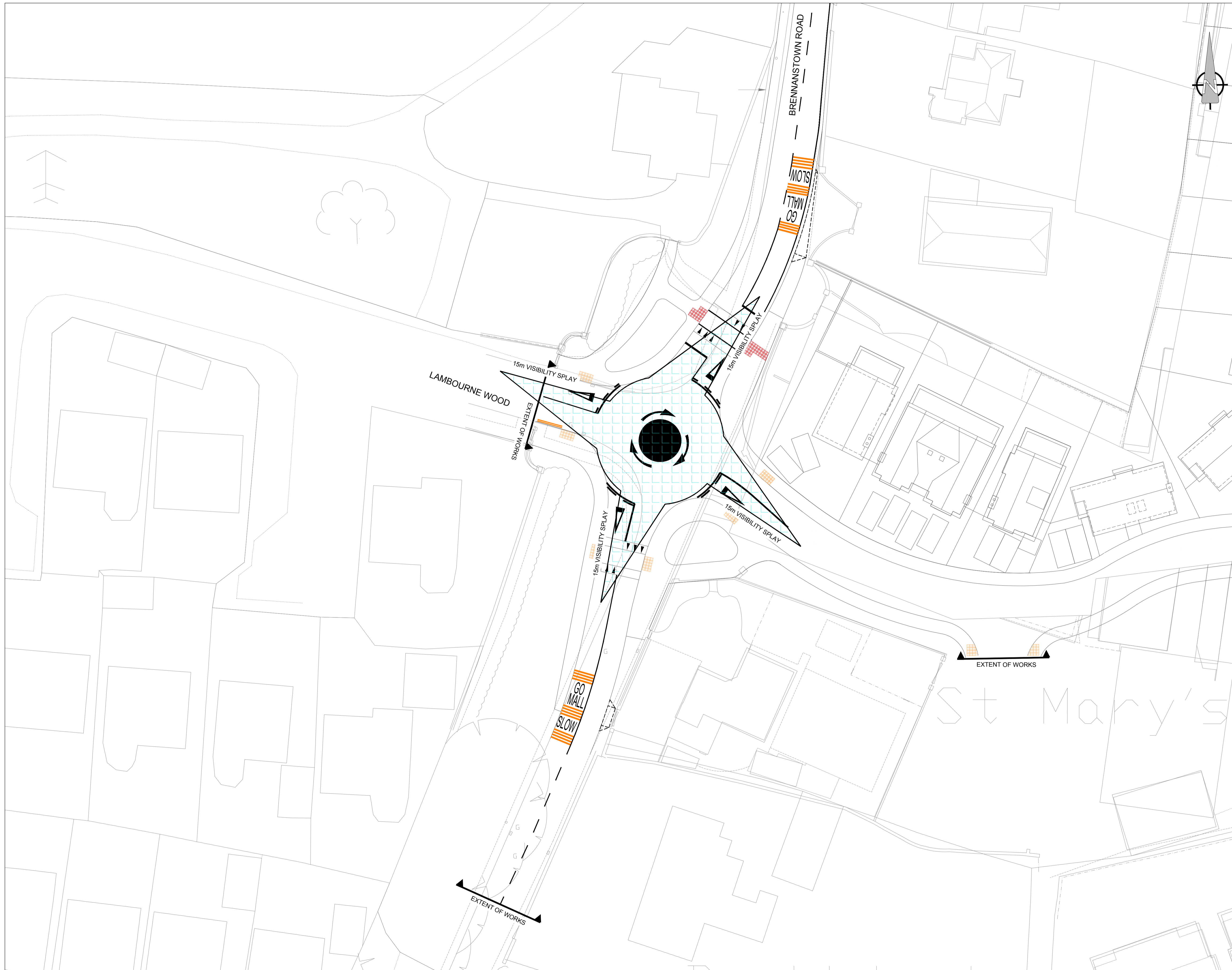
A PROPOSED ROUNDABOUT VISIBILITY SPLAY Scale: 1:250
